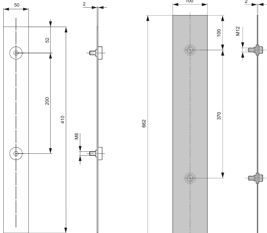
busbar covering PZ 00/100
