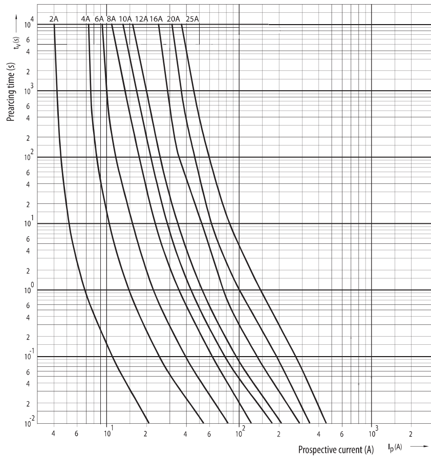
Time current characteristics
