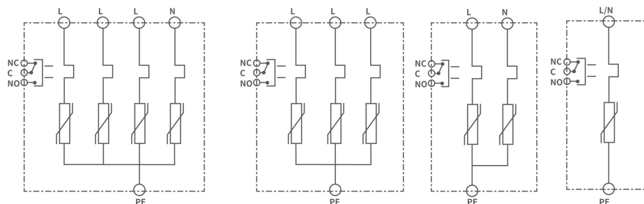
1. Alarm contact, 2. Thermal disconnecter, 3. Varistor
